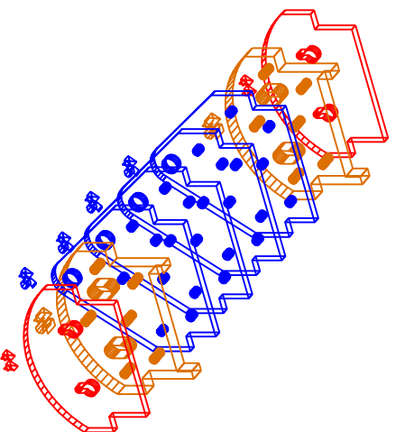
Exploded view of all the parts
